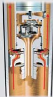
Left: Compression in 'Normal' mode – damper piston and bypass valve
