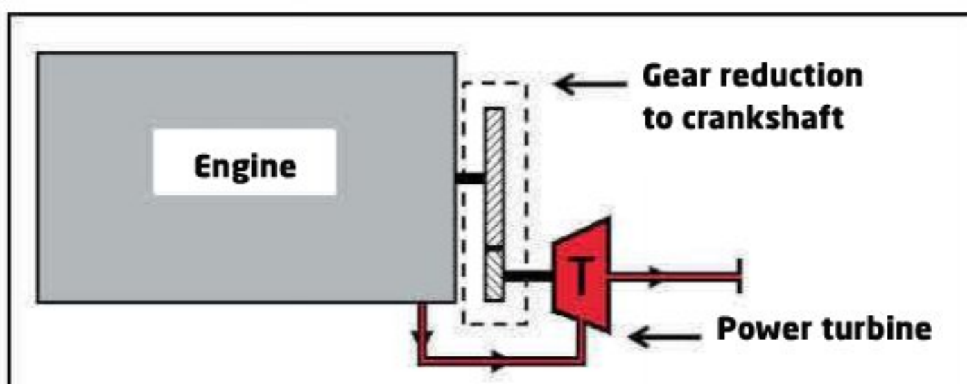
Figure 1: Basic turbocompounding
