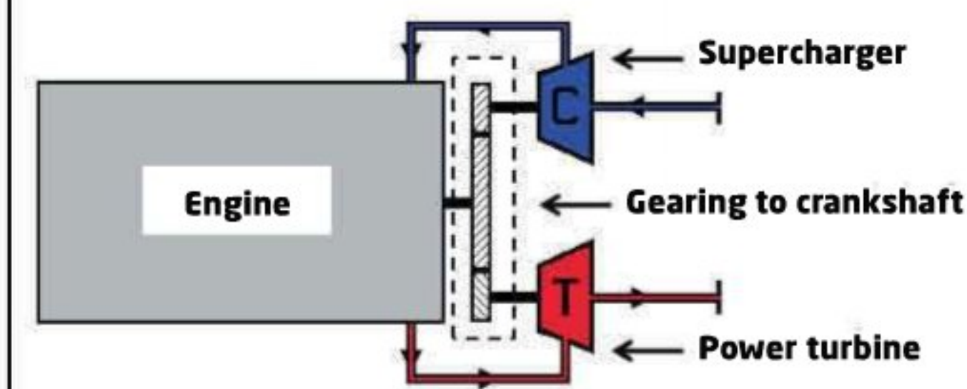
Figure 3: Supercharged turbo compound layout
