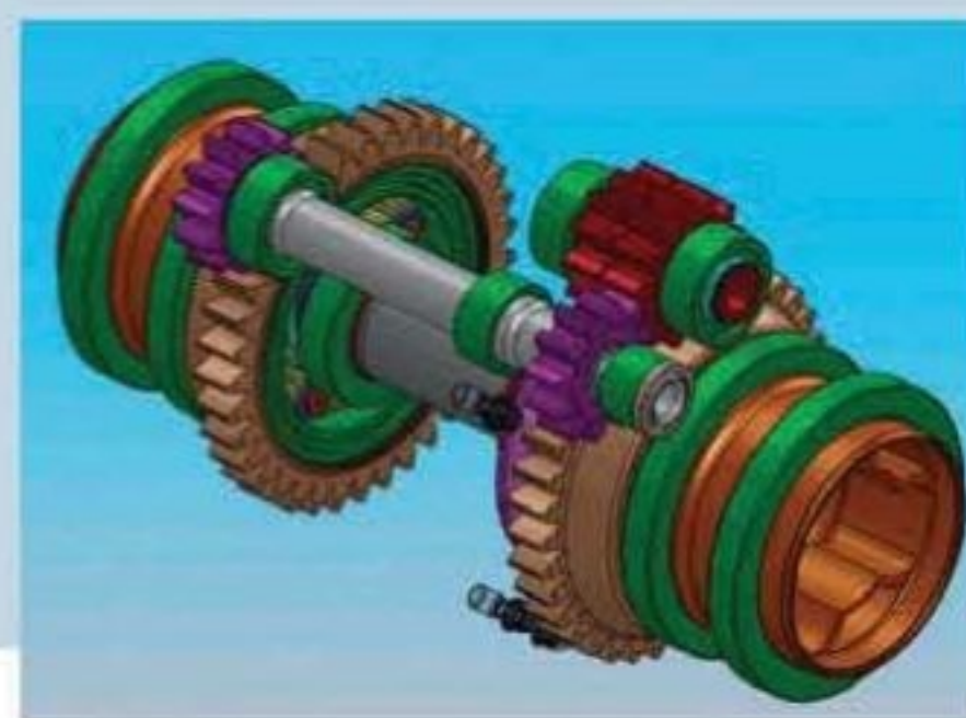
The DeltaWing transmission is a longitudinal unit with only five speeds. It is mounted in the conventional location and a manufacturer has been appointed though not yet named
