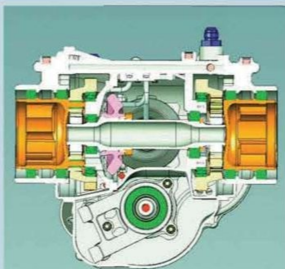
The DeltaWing transmission is a longitudinal unit with only five speeds. It is mounted in the conventional location and a manufacturer has been appointed though not yet named
