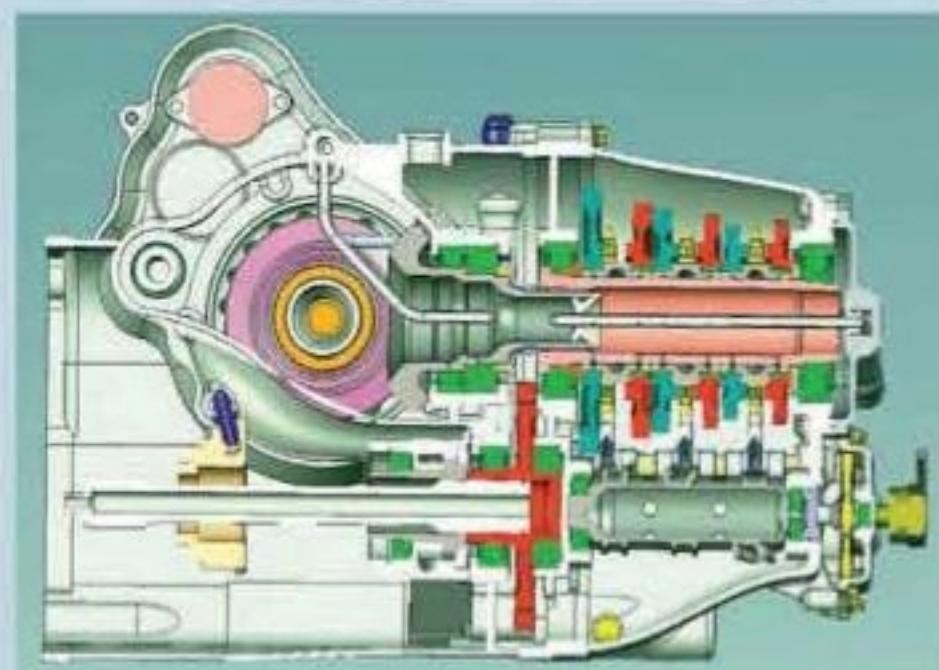
The DeltaWing transmission is a longitudinal unit with only five speeds. It is mounted in the conventional location and a manufacturer has been appointed though not yet named
