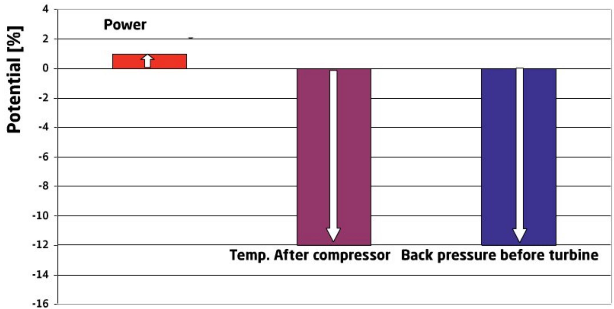
Compressor potential by optimised compressor impeller and housing
