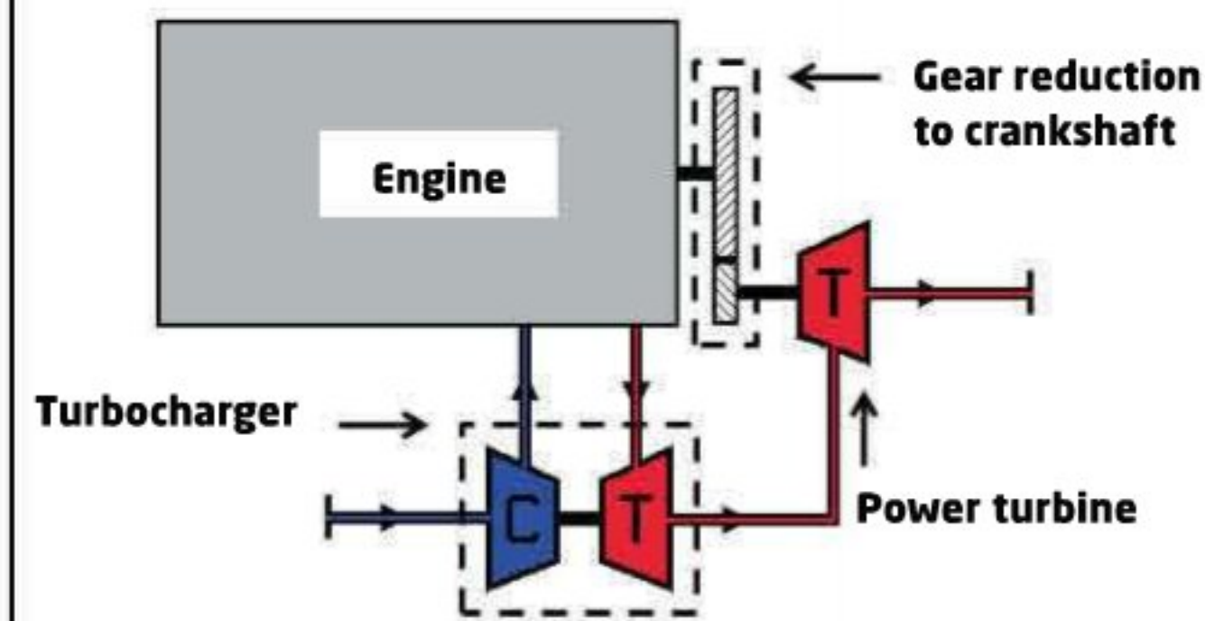
Figure 2: Turbocharged turbo compound layout
