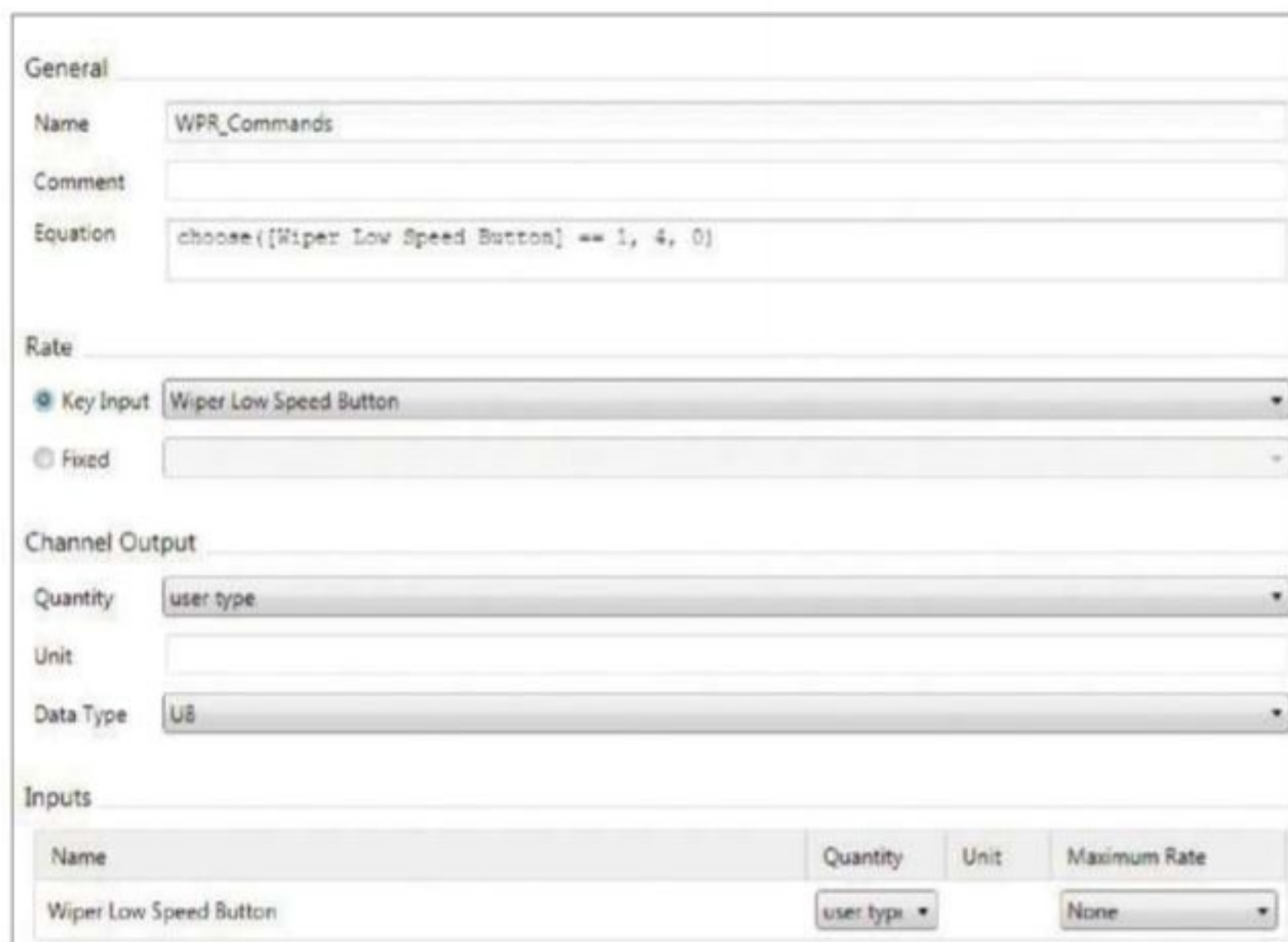
Figure 7: example of how a button press could be linked to a CAN control channel for a wiper motor
