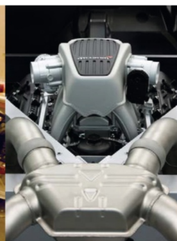
Left: McLaren's 3.8 litre V8 is the only GT3 car with a turbo engine Above: The lightweight MonoCell chassis is shared with the roadcar Left bottom: MP4 12C GT Sprint can be yours for £195,000
