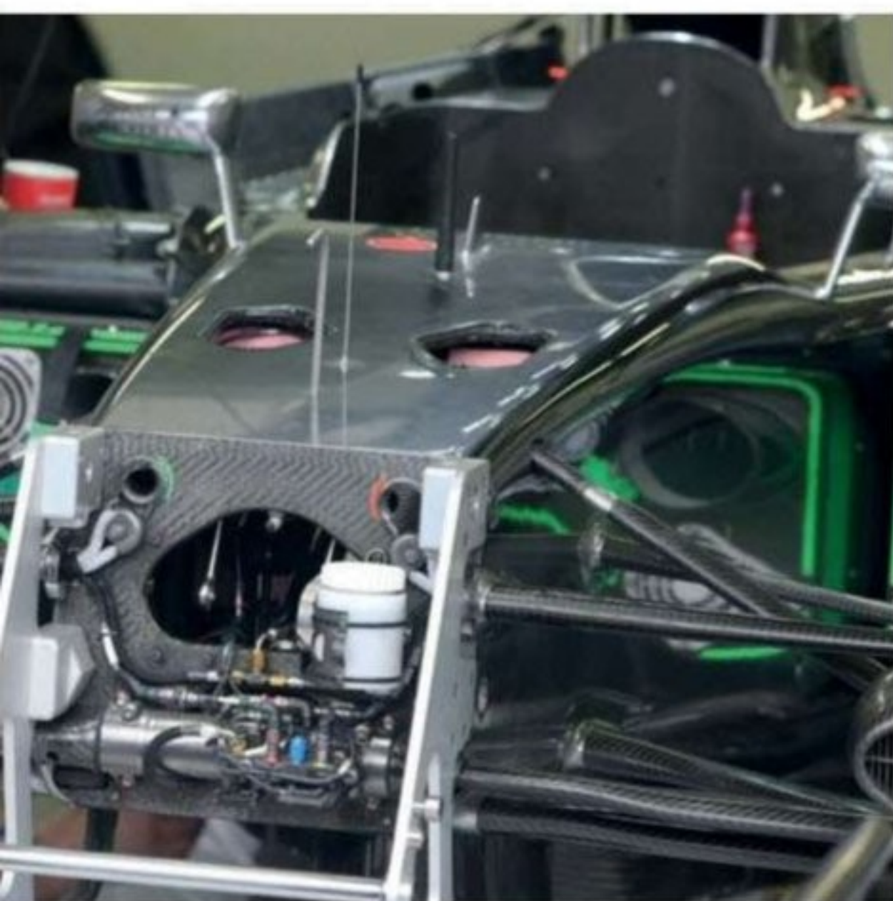
Partly disassembled, a pushrod end is visible through the bulkhead opening. This shot shows the front end without the FRICS hydraulics in place
