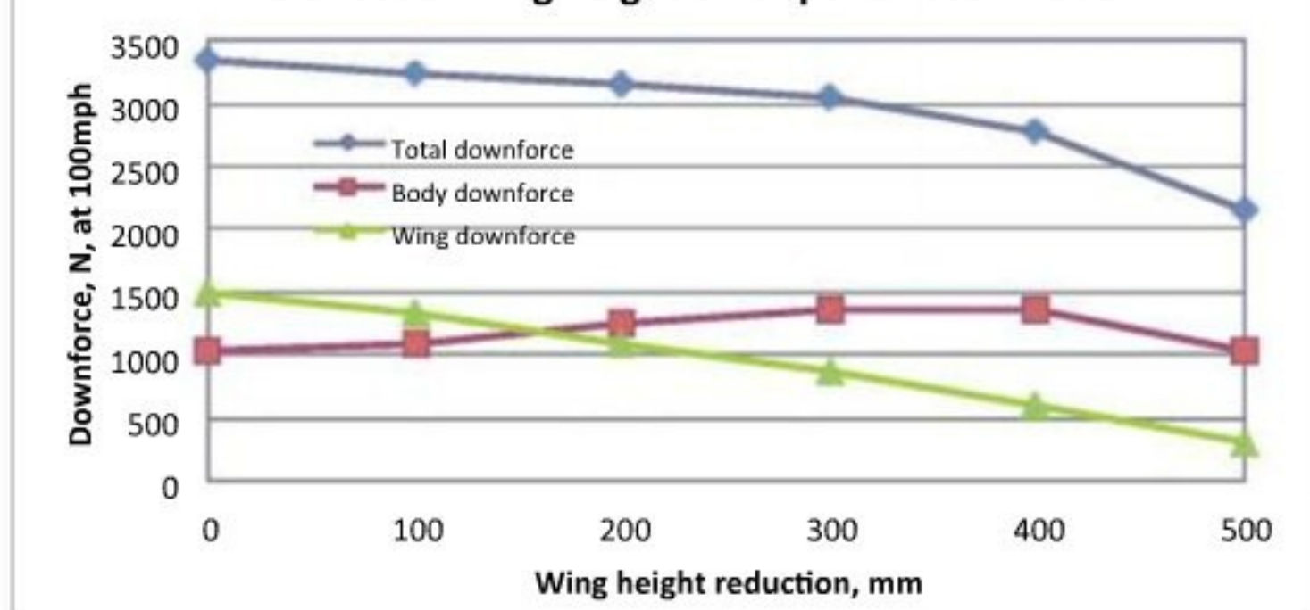
Figure 1: CFD-derived forces on a hillclimb sports libre model versus reduction in wing height
