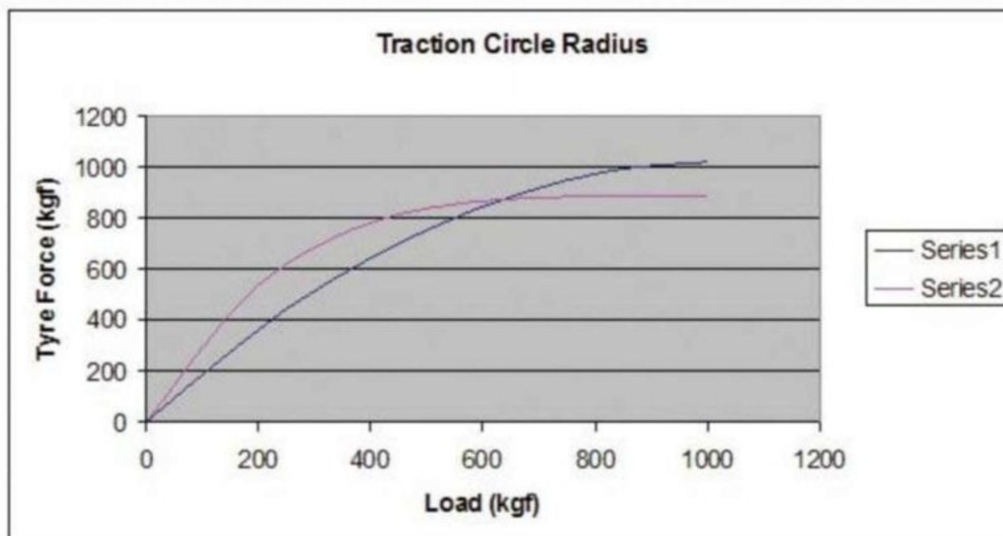
Figure 3: Plots of traction circle radius vs load
