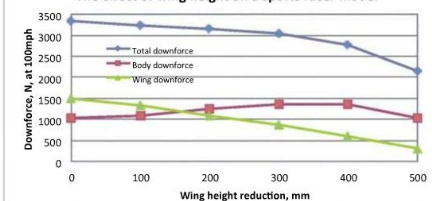
Figure 2: CFD-derived '%front' value on a hillclimb sports libre model versus wing height reduction
