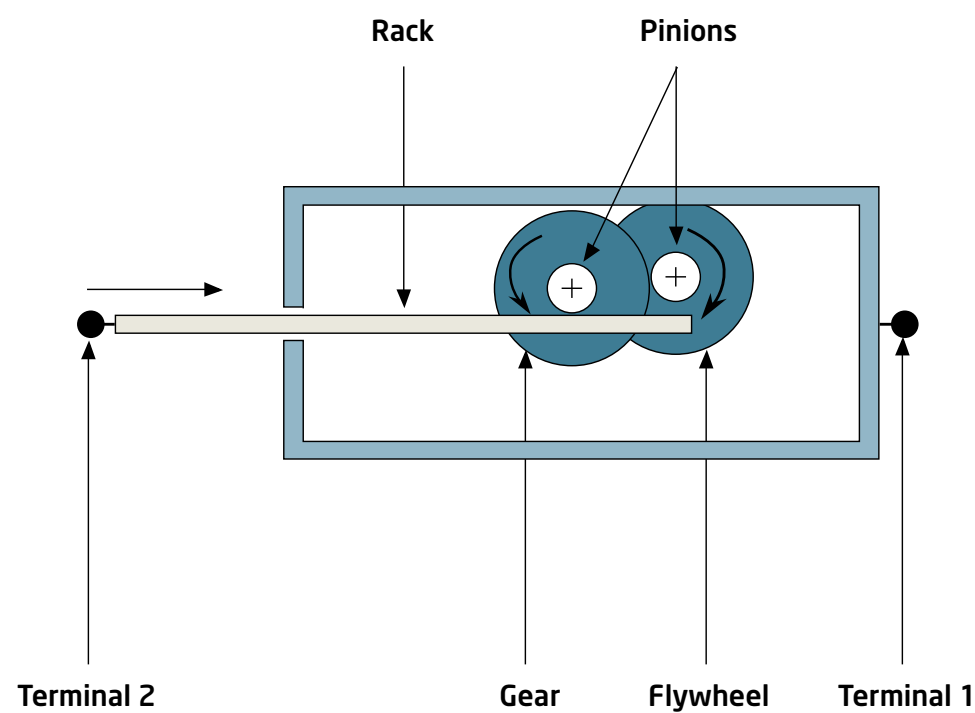
FIGURE 1 Mechanical interpretation of the principles of the inerter. One terminal is mounted on the casing, the other on a rack that drives a pinion as it moves in and out. The pinion drives a flywheel via a larger gear producing high rotational speeds and capturing large amounts of inertial energy compared to the mass of the whole unit
