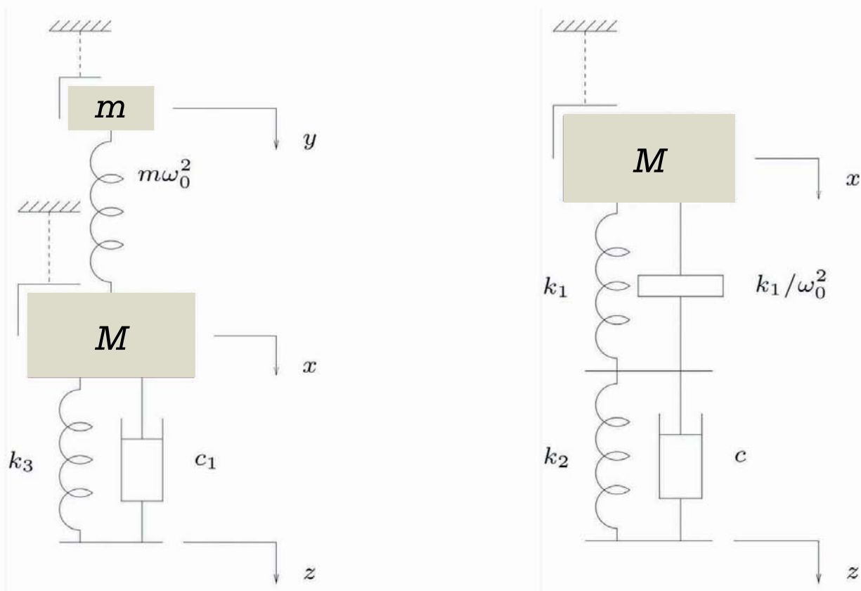
FIGURE 2 On the left is the normal arrangement of a mass damper ( m ) being used to stabilise a larger sprung mass ( M ). In contrast, the schematic on the right shows how an inerter is used to achieve the same effect
