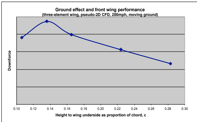
Figure 1: downforce from a front wing increases as ground clearance decreases - but only up to a point
