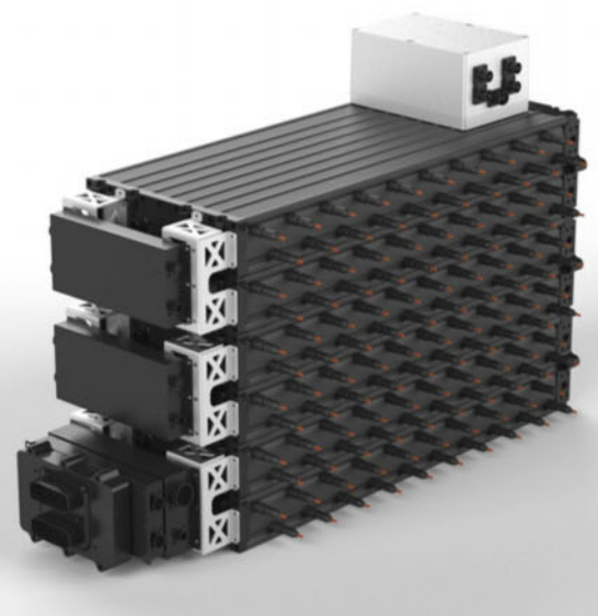
Left: Modular battery packs mounted in the floor of the Miss R car. Xing's approach allows for battery packs to be built up to suit the application and it is aimed at low volume electric vehicle projects Above: The Xing battery system is fully sealed and cooled by Novec fluid – a non-conductive liquid that has long been used for solvent cleaning, fire suppression and supercomputer cooling
