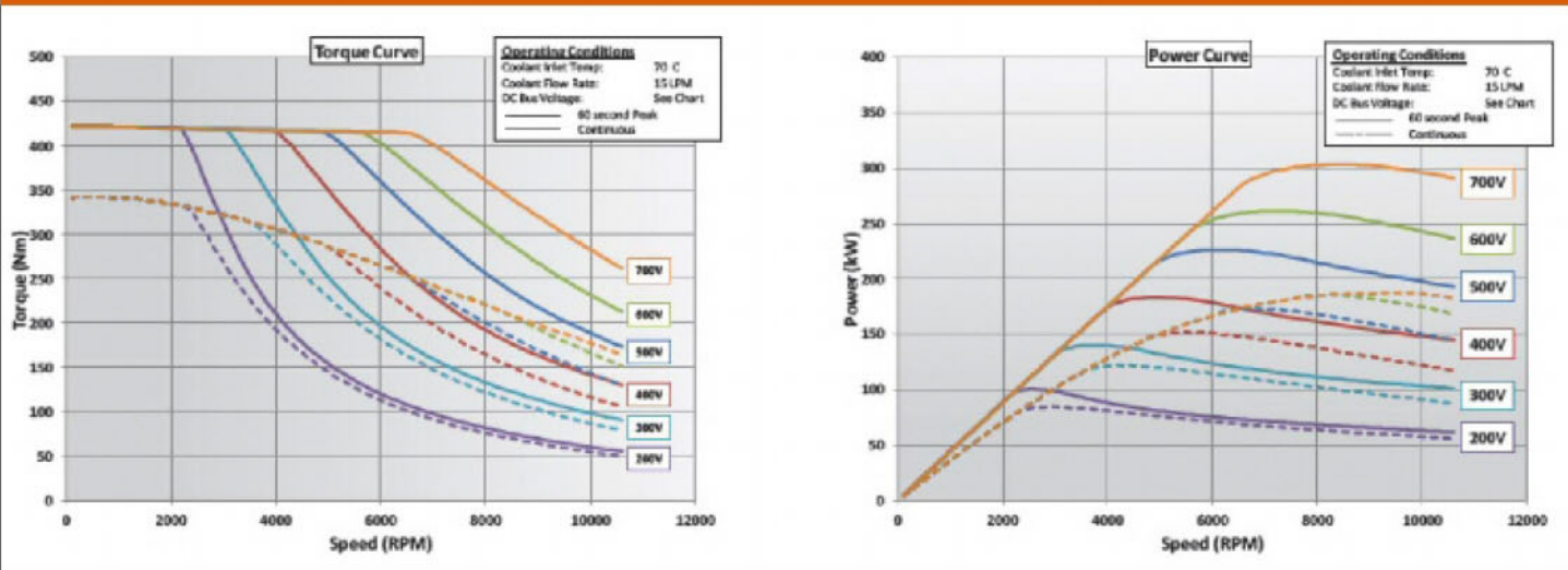
Figure 3: Electric torque curve for RPM and Voltage (courtesy of EV Systems Australia)
