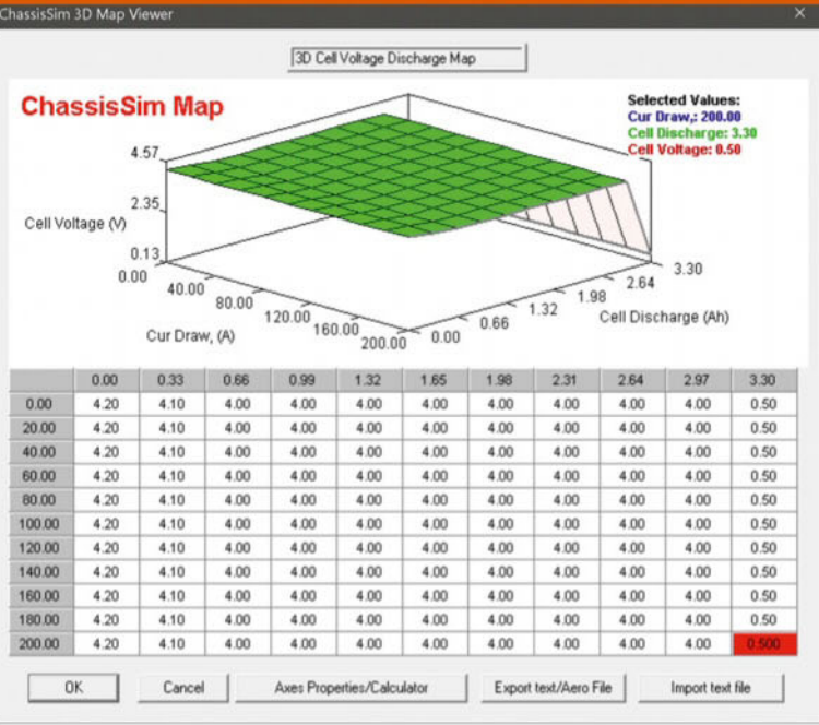
Figure 2: The perfect cell discharge curve
