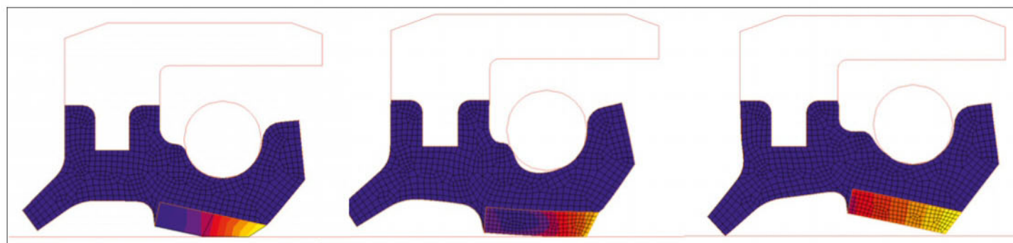
Left: The FEA analysis of wear of the PTFE contact lip Middle: Seal under positive pressure and pressing down on the shaft Right: Seal under vacuum lifting away from the shaft
