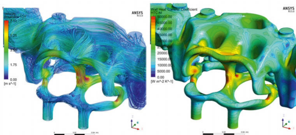
Left: Velocity streamlines showing flow of water around cylinder head Right: Distribution of wall heat transfer coefficient
