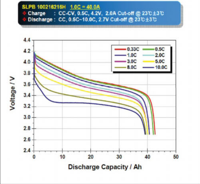
Figure 1: A sample of a cell discharge vs capacity and current for a high capacity cell
