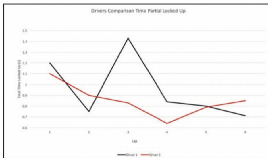
Figure 4: The driver lock-up trend across six laps. The data points to a car set-up issue
