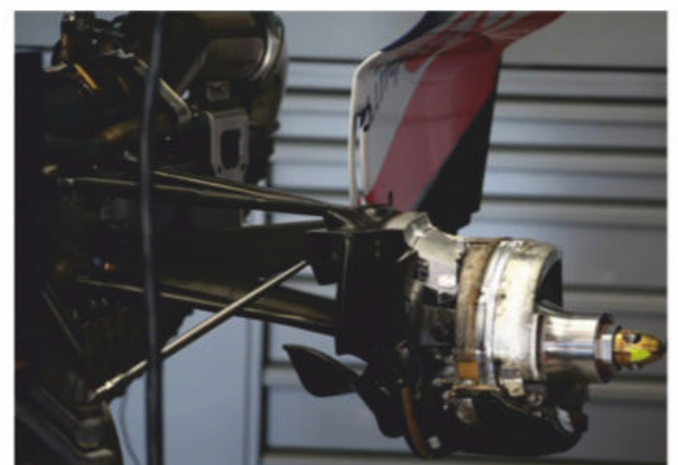
Rear suspension, brakes and uprights all come from the RB14
