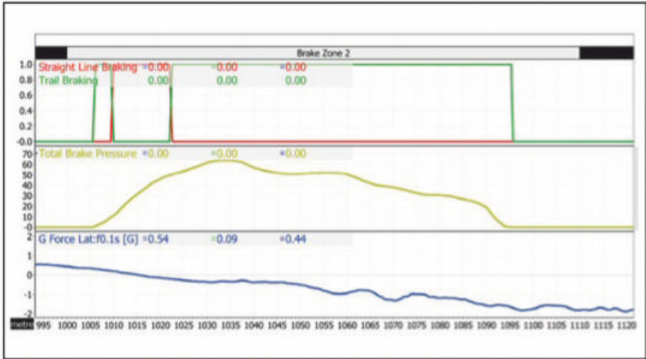
Figure 1: The red section corresponds to where the driver was within the bounds for straight line braking analysis, green is where it's within the bounds for trail braking
