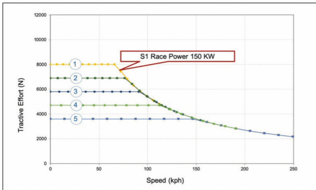
Figure 5: Thrust curves for the season one 5-speed gearbox. At around 100km/h you could use first, second or third gear
