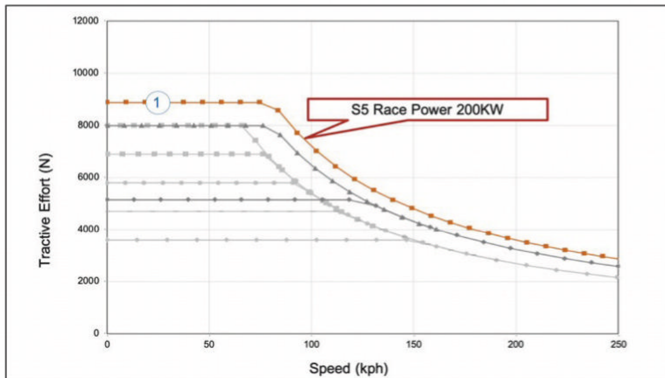
Figure 7: Motor thrust curves for season five. Power is up and single ratio gearboxes are now used by all the teams
