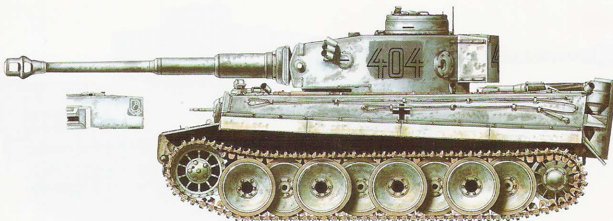
PzKpfw VI Sd Kfz 181 Ausf. H1 „Tiger“ z 4. kompanii 1. Pułku Pancernego SS, DGrenPanc. SS „LSSAH“, Charków, luty 1943 roku. PzKpfw VI Sd Kfz 181 Ausf. H1 “Tiger” of the 4th Company 1st SS–Panzer Regiment, SS–Panzer Grenadier Division “LSSAH”, Kharkov, February 1943.
