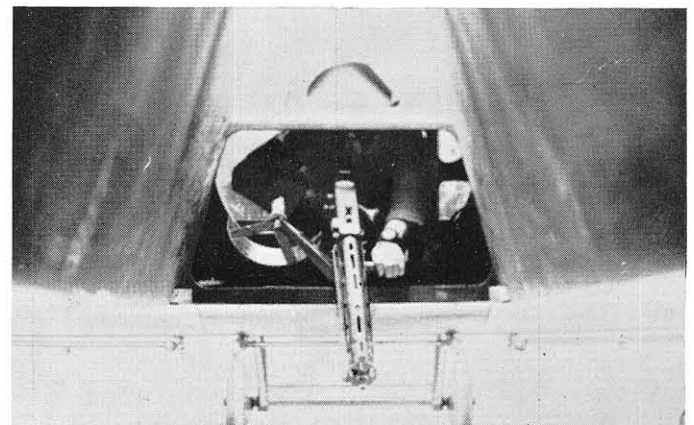
Looking forward along the gun-tunnel of a Gotha bomber. This enabled a pursuing fighter to be fired upon when supposedly in the 'blind-spot' position. Captain R. A. Little, a noted R.N.A.S. pilot was killed whilst attacking a similarly armed aircraft at night.
