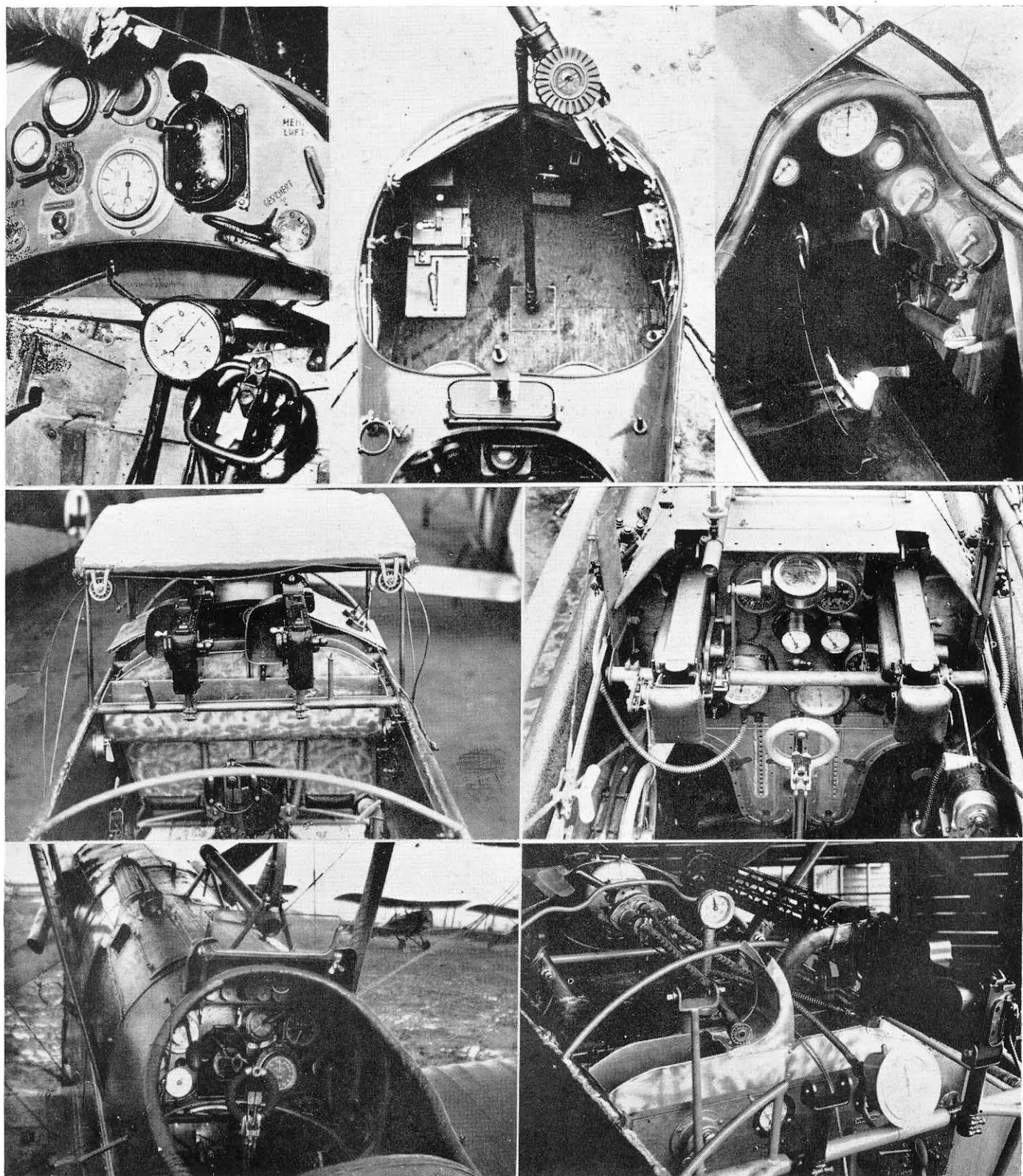
Top left: Hansa-Brandenburg D-1. Centre: Observer's cockpit on a F.E.2b; note additional gun mountings in front of pilot's cockpit. Right: S.V.A. Next: Fokker B-II (Austrian) and French-built 300 h.p. Dolphin Mark II. Bottom left: S.E.5a, probably of 56 Squadron; its long exhaust pipes have been replaced by short stubs. Note the Vickers gun and Aldis sight. Bottom right: Fokker D-VII. The left-hand gun has been temporarily removed.
