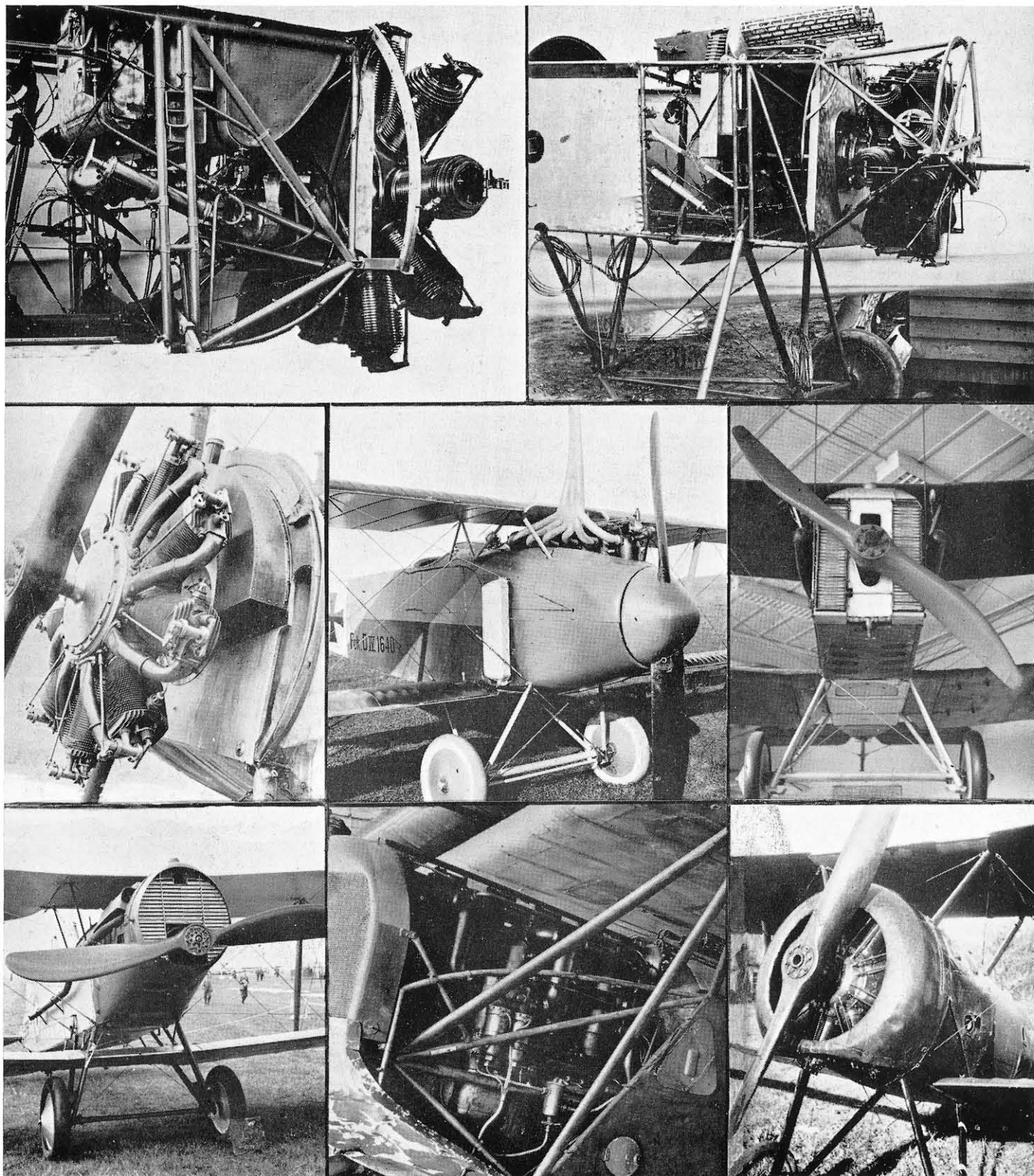
Top left: 100 h.p. Oberursel rotary on a Fokker E-II. Right: 160 h.p. double-row Oberursel fitted to Fokker E-IV 189/6, built for Immelmann. Next: 110 h.p. Le Rhône rotary of a Nieuport 12; a modified Fokker D-IV and a Viper-engined S.E.5a. Bottom: Bristol F2B; Fokker D-VII (O.A.W.) 4635/18 in the Smithsonian Institute, U.S.A. (flown by Lieutenant Heinz von Beaulieu-Marconnay, brother of the German ace) and a B.R.2 powered Snipe.
