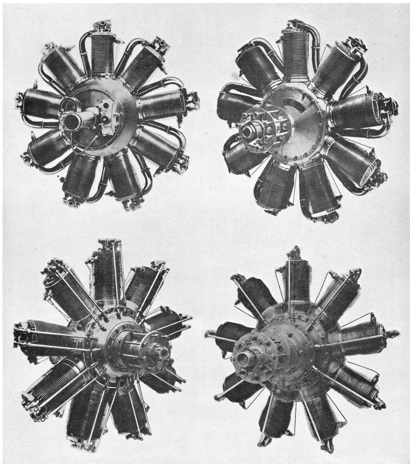
Top Left: 80 h.p. Le Rhône (rear view) bore/stroke 105 × 140 mm. Top Right: 110 h.p. Le Rhône bore/stroke 112 × 170 mm. Bottom Left: 130 h.p. Clerget bore/stroke 120 × 172 mm. Bottom Right: 100 h.p. Gnôme-Monosoupape bore/stroke 110 × 150 mm.
