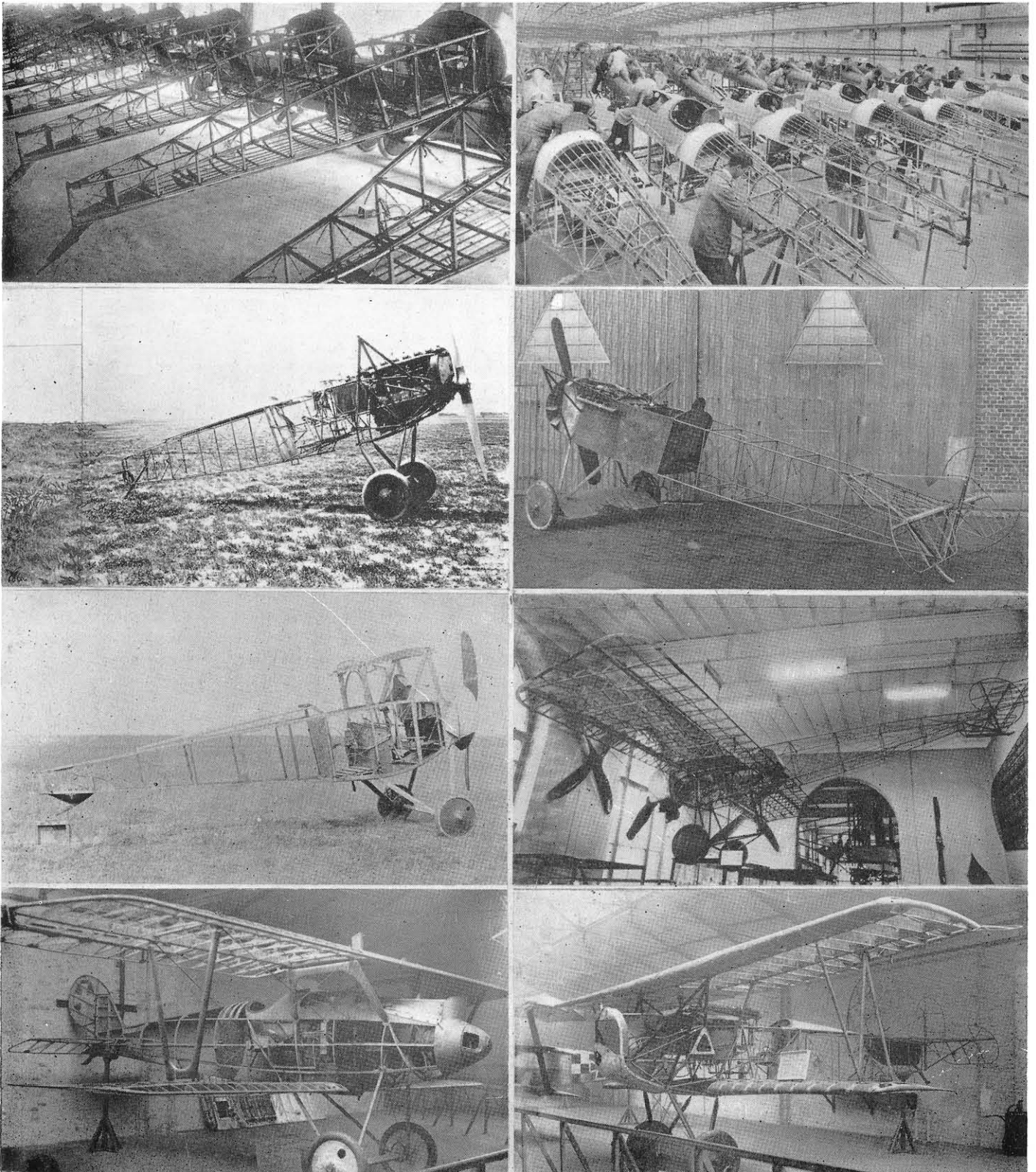
Left: American—Thomas Morse Scouts—wood. German—Fokker D-VII—metal. French—Nieuport 10, two-seater—wood. German—Pfalz D-IIIa—wood. Right: British—S.E.5s at the Wolseley factory—wood. German—The experimental Fokker V-37 monoplane with armoured Mercedes engine and cockpit—metal. German—Fokker Monoplane—metal. German—Fokker D-VII—metal. (Note Stapenhorst's chequered triplane behind the D-VII.)
