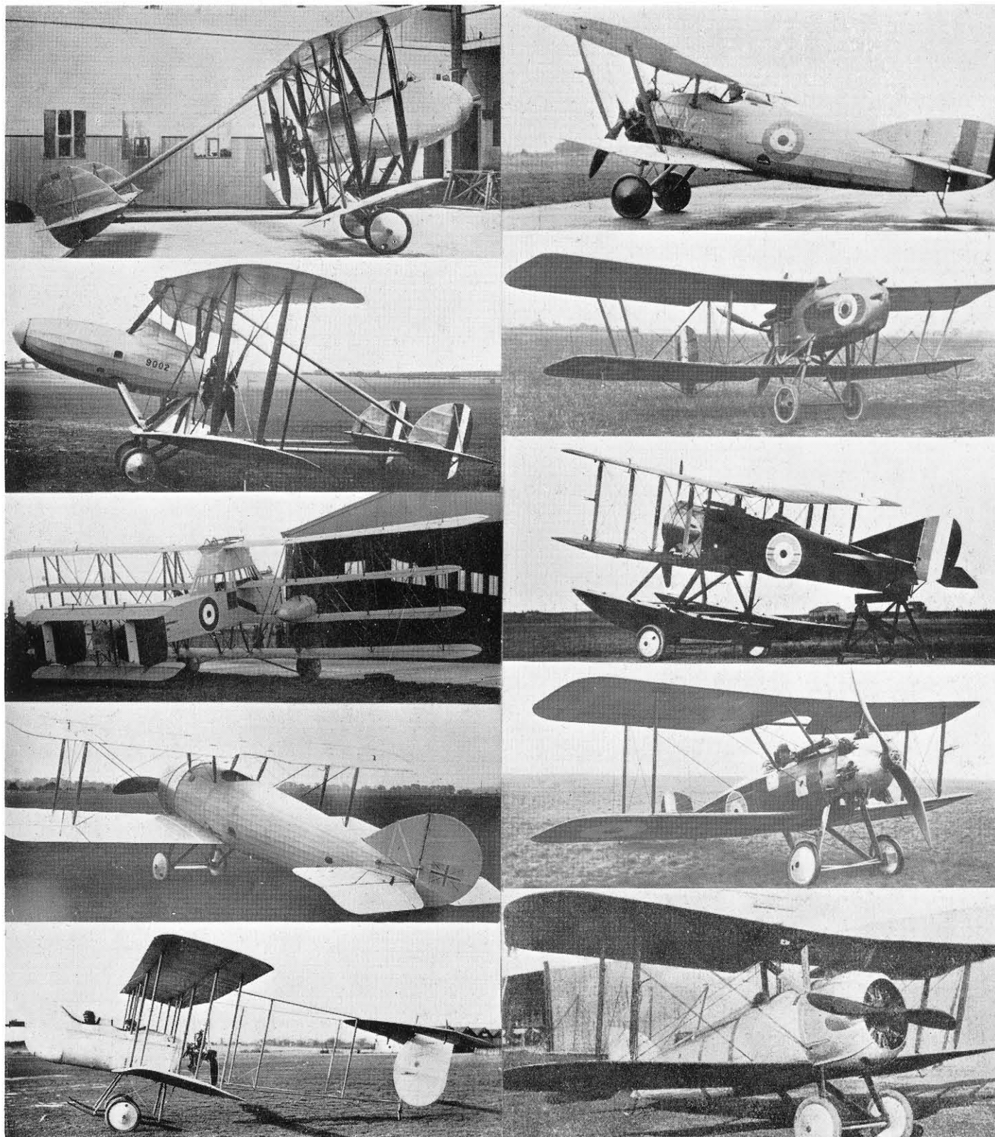
Left—Top to Bottom: Pemberton-Billing P.B.23. 80 h.p. Le Rhône. The original 'Push-Proj.' Pemberton-Billing P.B.25. 100 h.p. Gnome Monosoupape, 1915. Supermarine Nighthawk 2 x 100 h.p. Anzani Anti-Airship Fighter, 1915-1916. Vickers E.S.1. 100 h.p. Gnome Monosoupape, 1915. Vickers Fighting Biplane. 100 h.p. Gnome Monosoupape. Forerunner of the 'Gun-Bus', 1914. Right—Top to Bottom: Vickers F.B. 16. 150 h.p. Hart. An early version, 1916. Vickers F.B.26. 200 h.p. Hispano-Suiza with Eeman triple gun mounting, 1917. Westland N.1B (Serial N-17). 150 h.p. Bentley B.R.1. Fighter Seaplane, 1917. Its predecessor, N-16, differed in having Sopwith-type main floats and a tail float. Both 1917. Westland Wagtail. 170 h.p. A.B.C. Wasp I. Original version, 1917-1918. Whitehead Scout. 80 h.p. Le Rhône, 1916.
