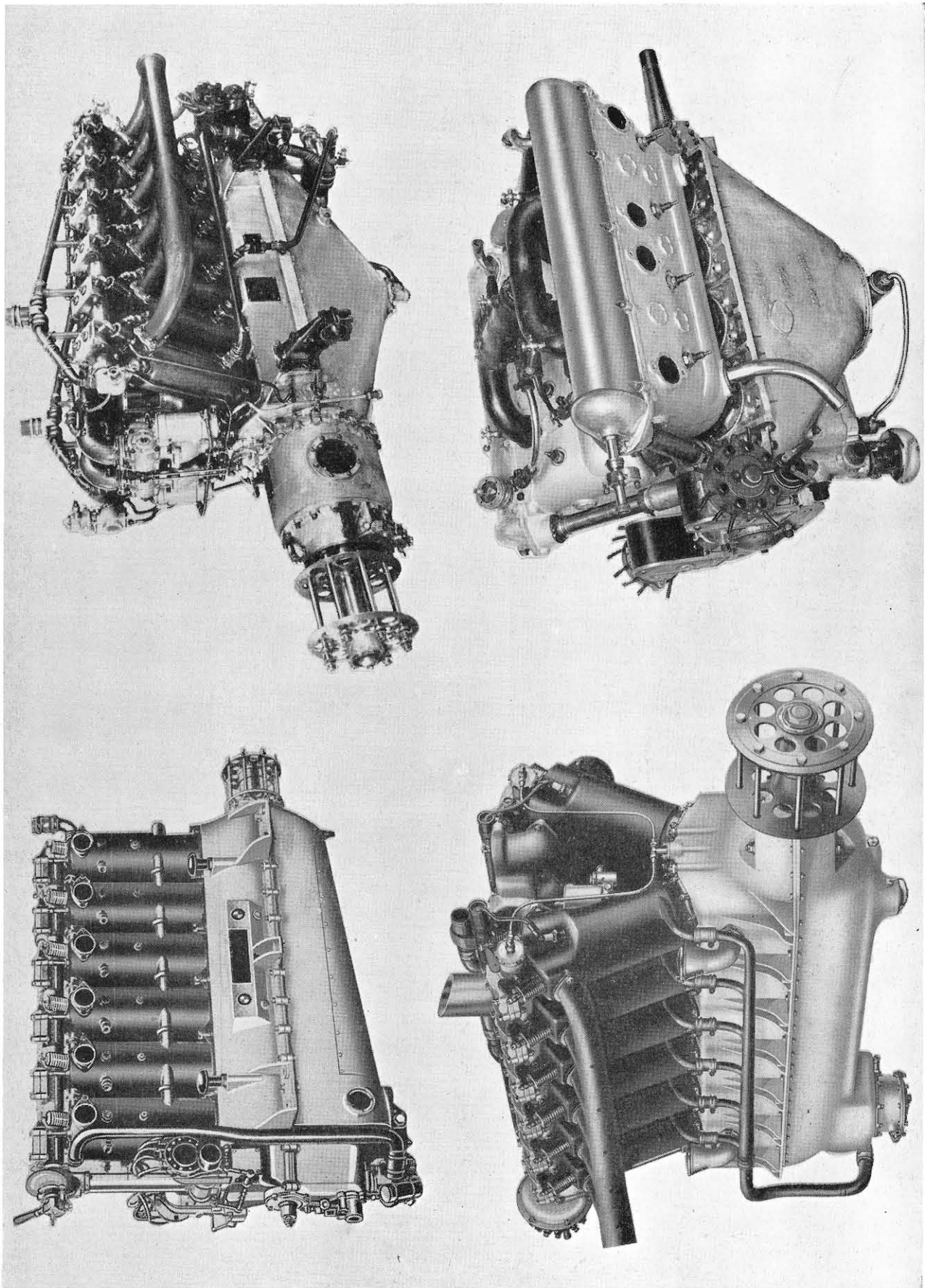
Top Left: 185 h.p. B.M.W. bore/stroke 120 × 150 mm. Top Right: 275 h.p. Rolls Royce 'Falcon II' bore/stroke 4" × 5 3/4". Bottom Left: 400 h.p. Liberty bore/stroke 127 × 177.8 mm. Bottom Right: 200 h.p. Wolseley 'Viper' 4.72" × 5.12".
