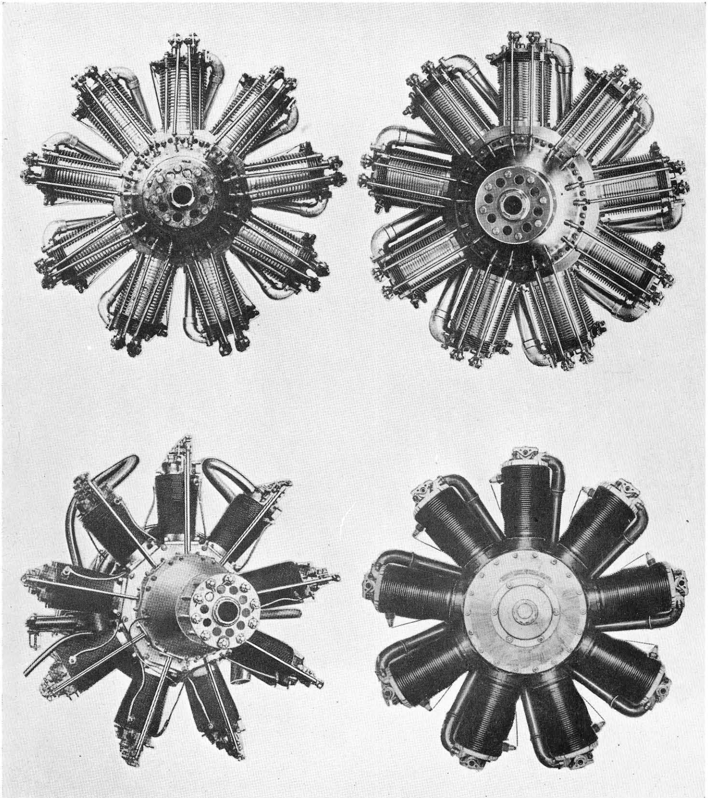
Top Left: 150 h.p. Bentley B.R.1 bore/stroke 120 × 170 mm. Top Right: 200 h.p. Bentley B.R.2 bore/stroke 140 × 180 mm. Bottom Left: 320 h.p. A.B.C. Dragonfly (Radial) bore/stroke 140 × 160 mm. Bottom Right: 110 h.p. Oberursel UR.II bore/stroke 112 × 170 mm.
