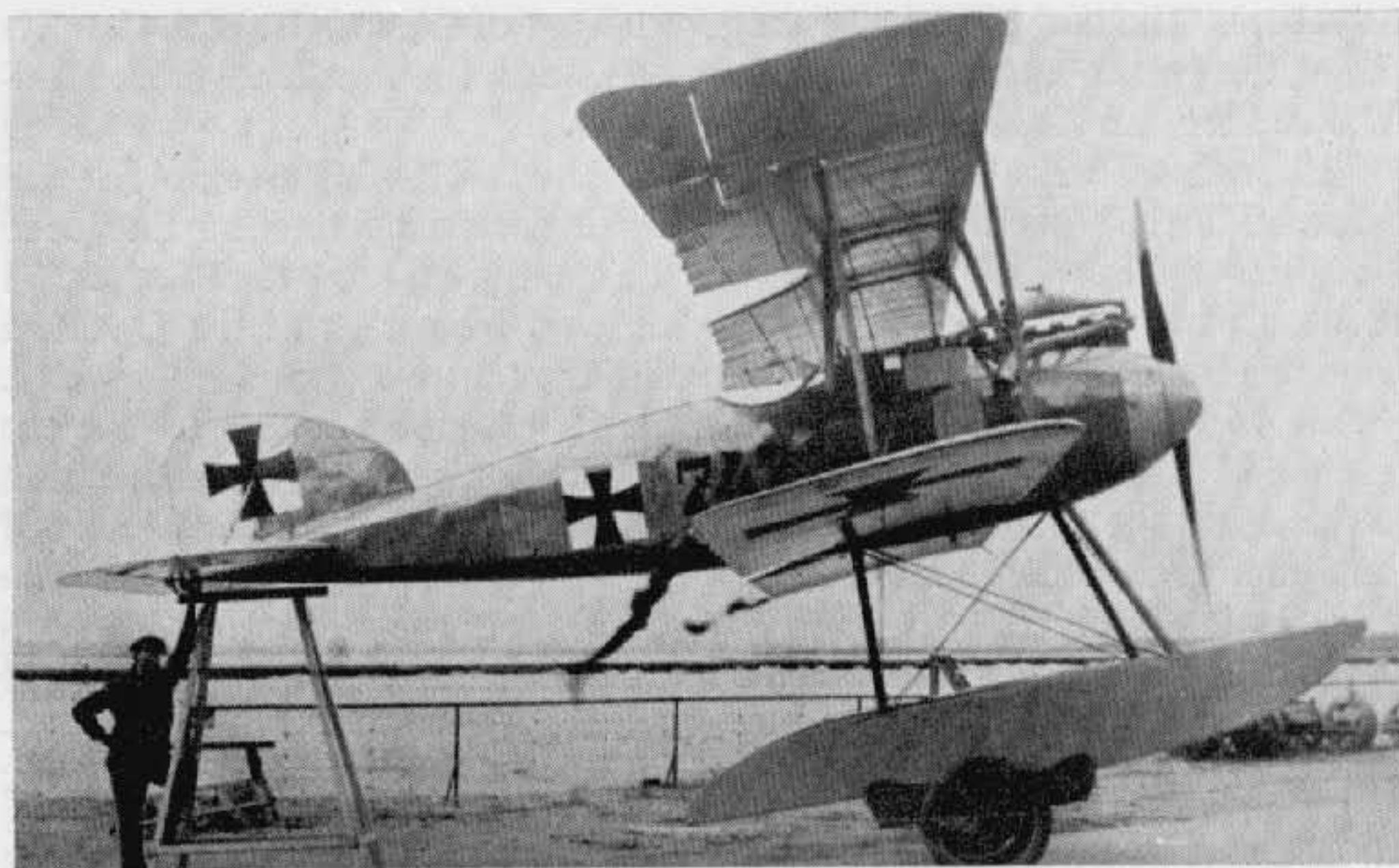
Albatros W 4 (Marine number 747). (Photo: Real Photographs Co. Ltd.)
