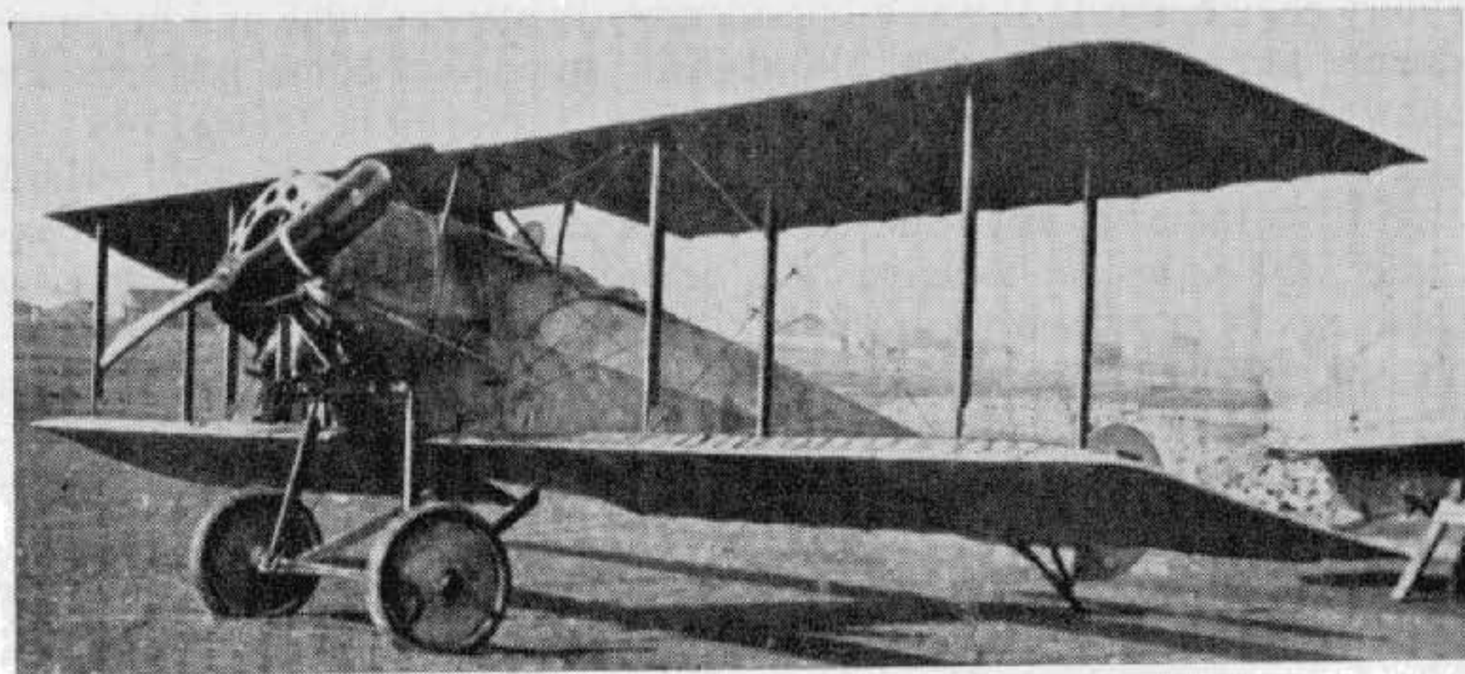
Fokker D III. (Photo: Real Photographs Co. Ltd.)
