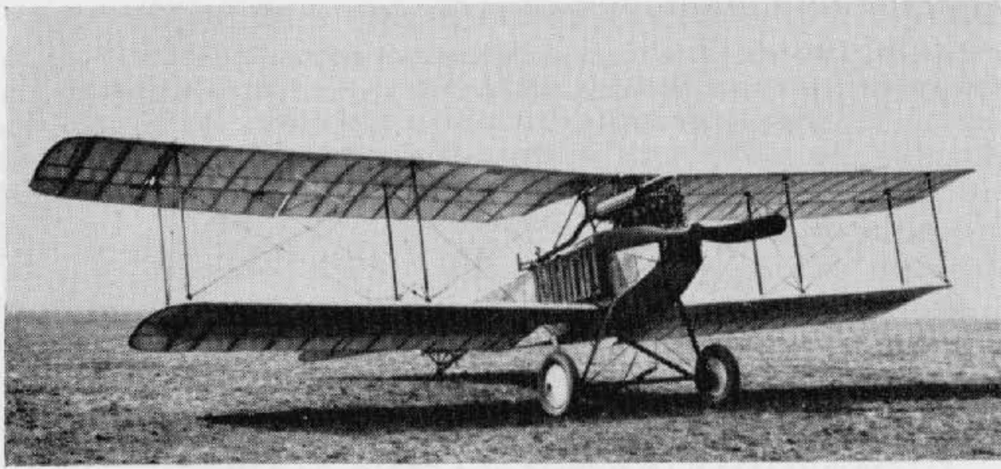
Albatros C I (160 h.p. Mercedes with long exhaust pipe). (Photo: Imp. War Museum.)
