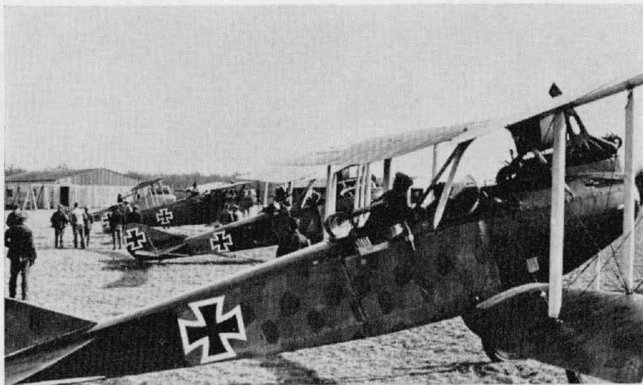
An interesting collection of two-seaters, typifying the equipment of 1917-18. In the foreground is a Rumpler C IV, the other aircraft being a Rumpler C VII, a Hannover CL IIIa and a D.F.W. C V. (Photo: A. Imrie.)
