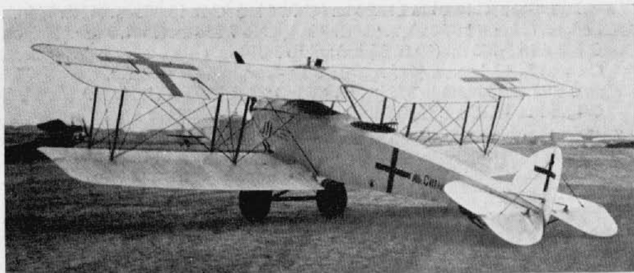
Albatros C III (licence-built by D.F.W. with modified fin and rudder). (Photo: A. Imrie.)
