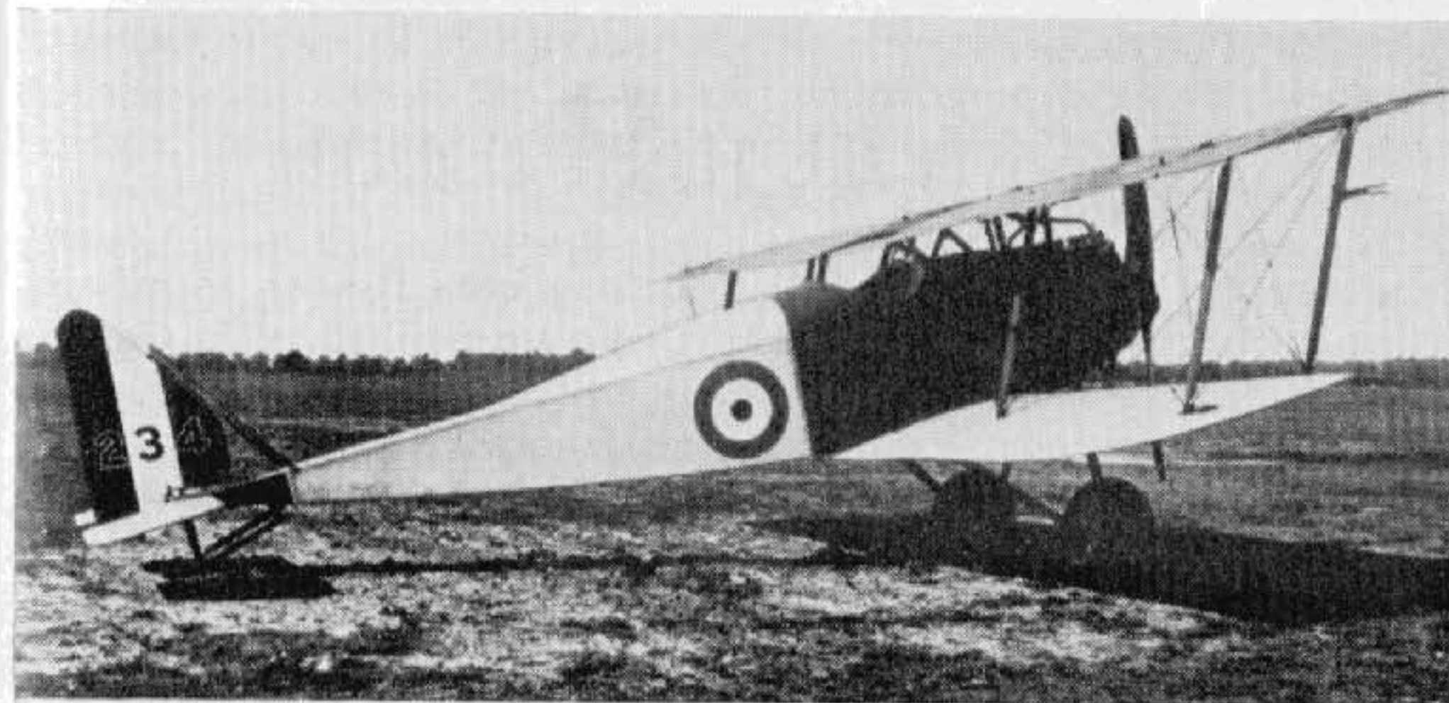
Halberstadt D III captured by the R.F.C. and given British roundels. (Photo: Aero Modeller.)
