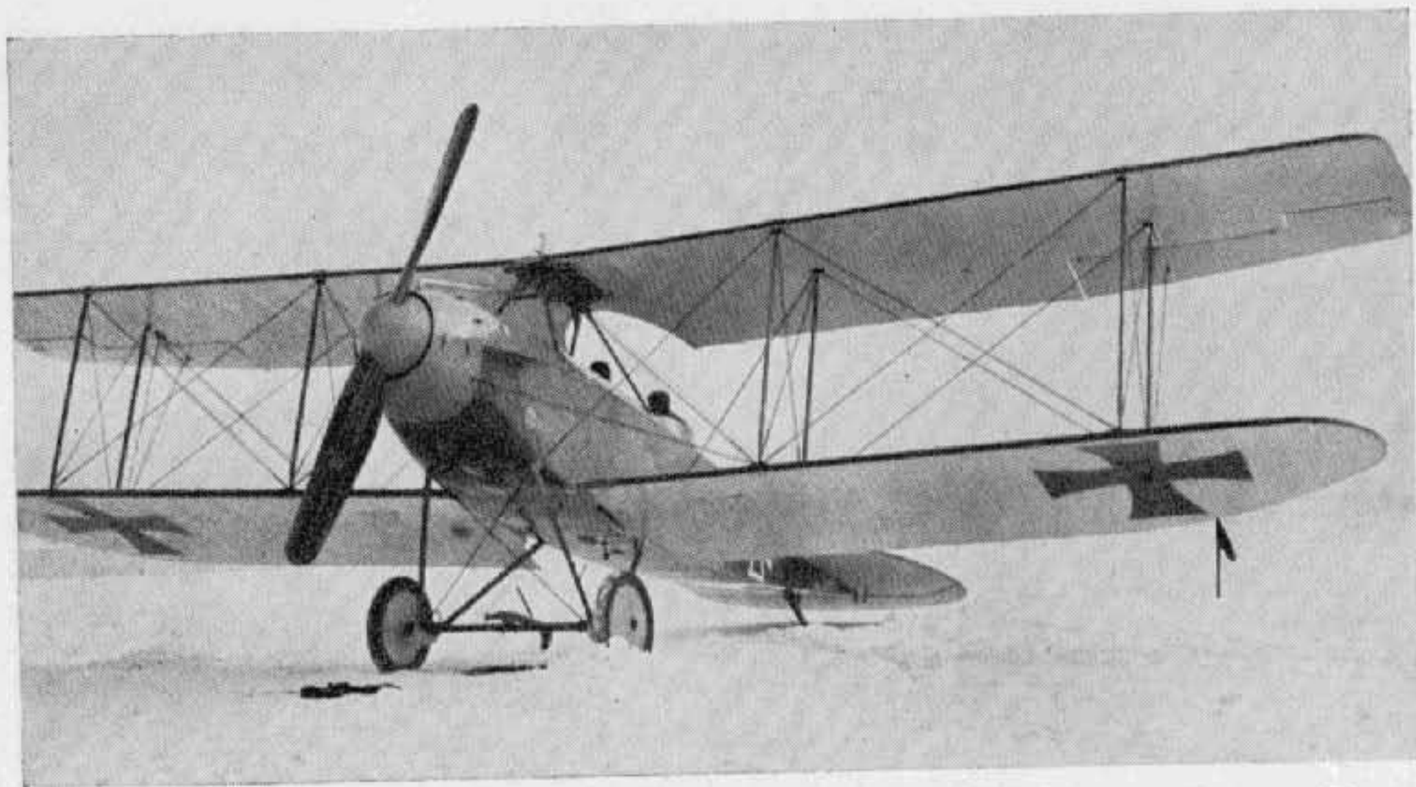
Albatros C V/17, with curved lower wing and balanced control surfaces. (Photo: A. Imrie.)
