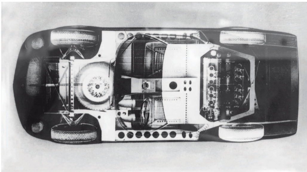
The Miura's compact steel monocoque "tub" was advanced compared with Lamborghini's competitors—Ferrari included—and featured strategically located holes to lighten the structure.
