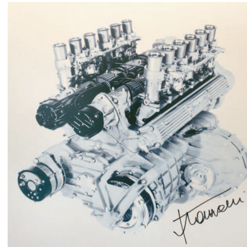
The Miura's engine and transmission were cast as one piece in aluminum, and early models had a single sump.
