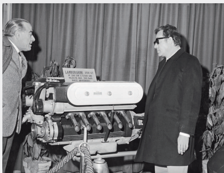
Gian Paolo Dallara modified the power curve of the prototype V-12 and added a wet sump; horizontal carburetors enabled it to fit beneath the 350GT's low hood.
