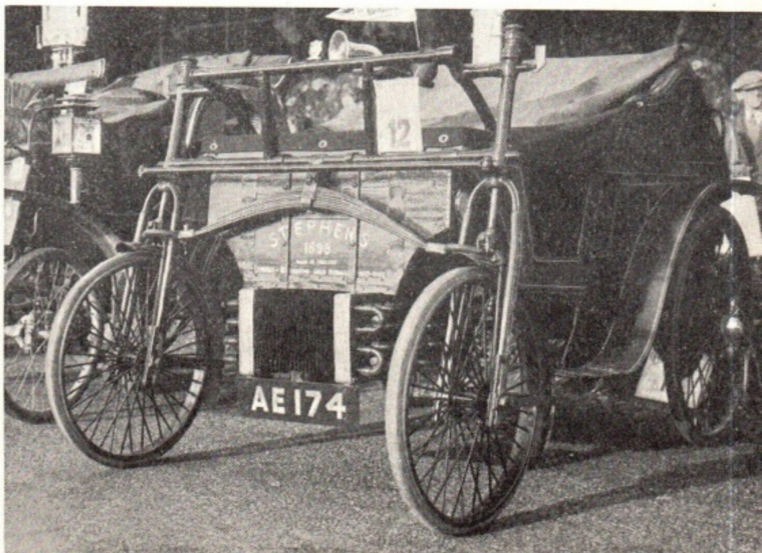
INDEPENDENT: (Below). I.f.s. as featured on the 1898 Stephens which took part in the 1950 R.A.C. Veteran Car Run.
