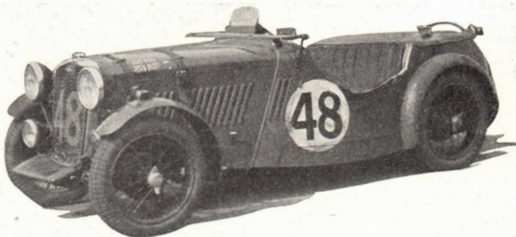
PROGENITOR —This was the Singer "Nine Sports" as modified for the Le Mans race, 1933. The rear seating space was occupied by a large fuel tank as is evident by the filler caps. From this car was evolved the two-seater Le Mans model.
