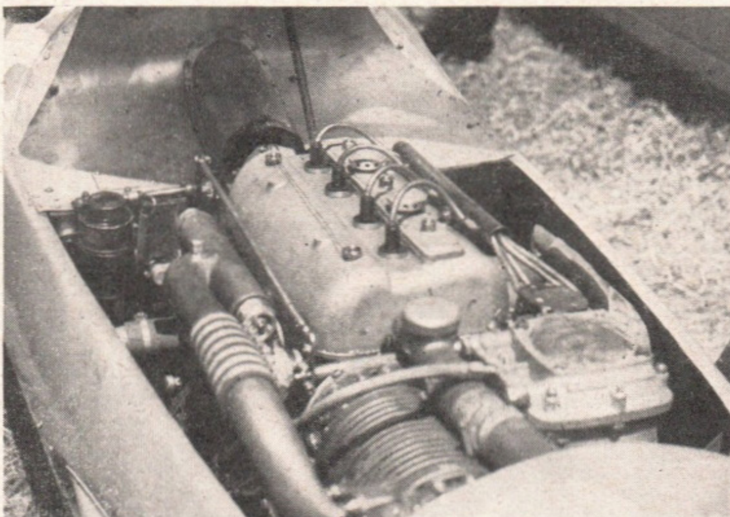
BLOWN SIMCA: An under-bonnet view of the Wade-blown 1½-litre 4-cylinder Simca engine, the type with which Maurice Trintignant won last Sunday's Albi G.P.
