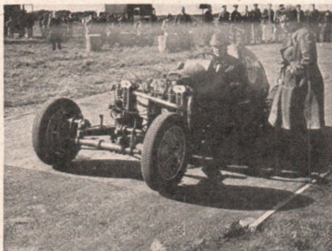
TWO SINGLES TO ALTCAR: Charlie Oates in the remarkable Murray Special with two 500 c.c. J.A.P. engines mounted side by side. It scored a "second" in its class.
