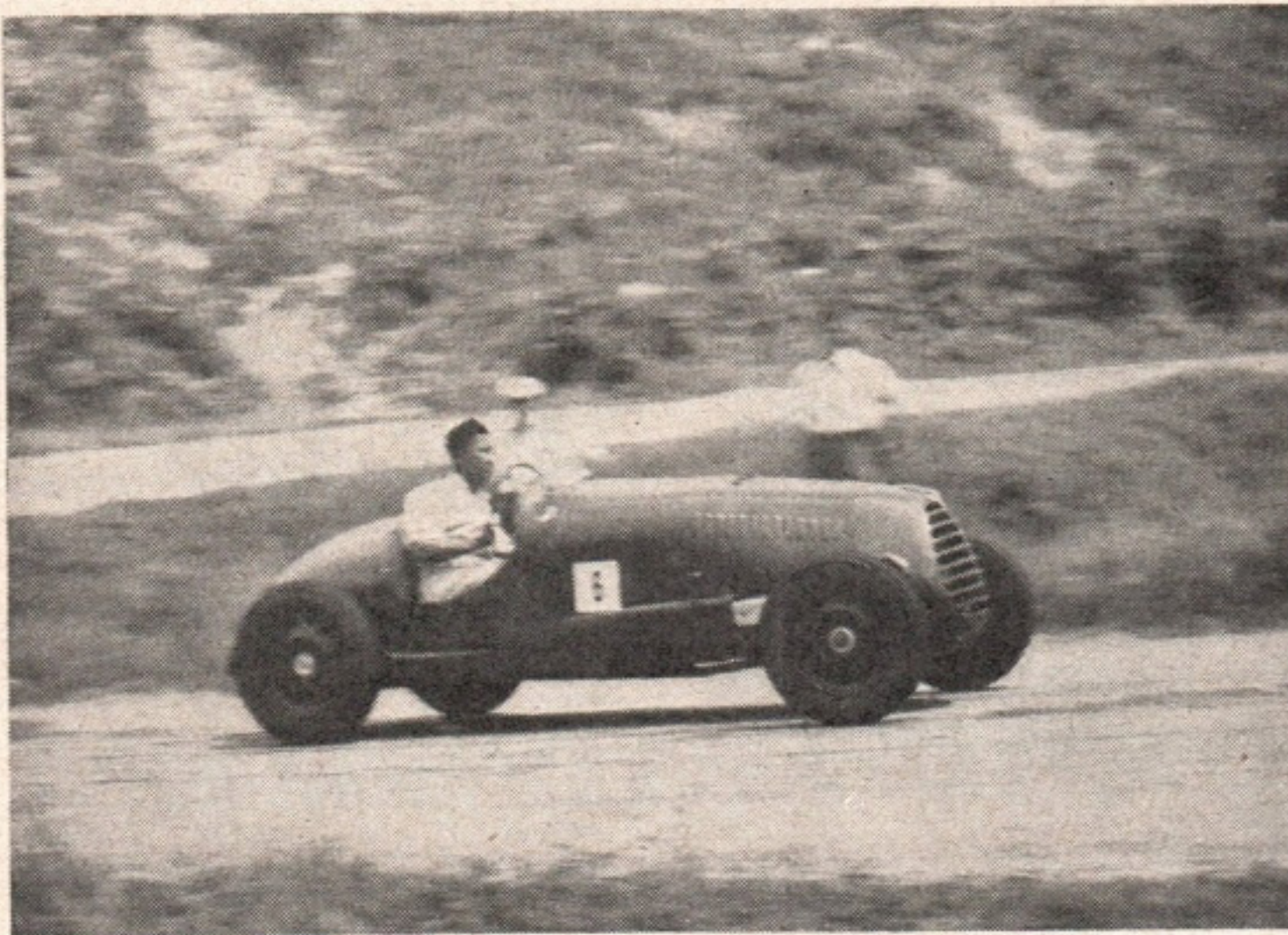
EFFECTIVE MIXTURE: The Airhen Special with Jowett Javelin engine in a Fiat 1,100 chassis, and neat single seater bodywork reminiscent of a Cisitalia. Driven in the Singapore M.C.'s recent Gap Hill-climb by Chia Eng Quee, it secured a second place in the 1,500 c.c. racing class.
