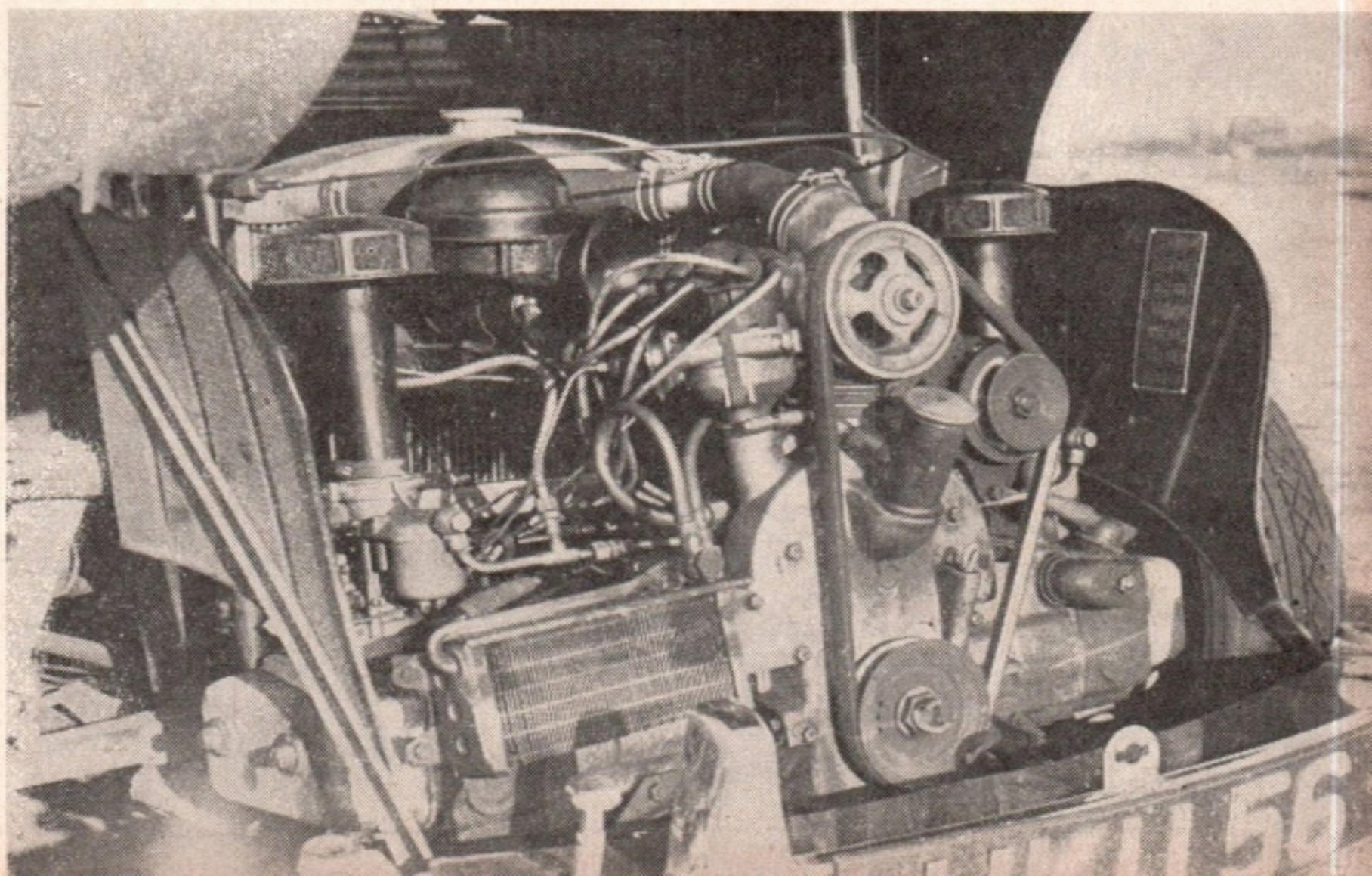
FLAT FOUR: (Right) . . . or more correctly, horizontally opposed 4-cylinder—a close-up of the efficient Jupiter o.h.v. engine, showing the oil cooler, water-pump and dynamo drive, distributor and the "mushroom" pattern air-silencers for the two Zenith down-draught carburetters.
