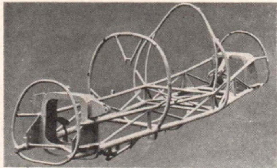
500 cc. Frame supplied to Mr. Ken. Smith, winner of the non-series production 500 cc. race at Silverstone, 1951
