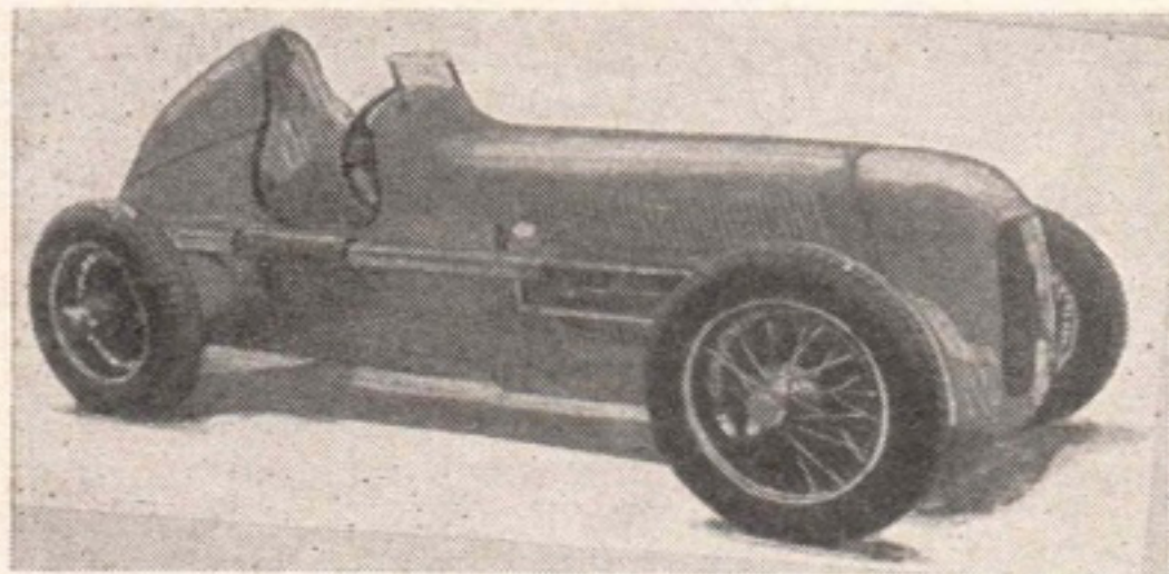
The 1½-litre 6-cylinder supercharged two-stroke Zoller, designed by Dr. Arnold Zoller and built in 1934. Its appearances in racing were few and unsuccessful.
