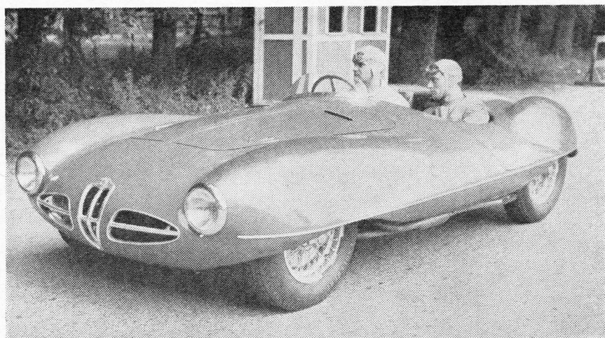
LE MANS ABSENTEE: Alfa Romeo's sensational new competition sports-car, called the "Disco Volante" (Flying Saucer), seen at Monza with Sanesi at the wheel. The engine is a six-cylinder of 82.5 mm. x 90 mm. bore and stroke (2.9 litres). Superleggera bodywork is by Touring, and weight is under 15 cwt.
