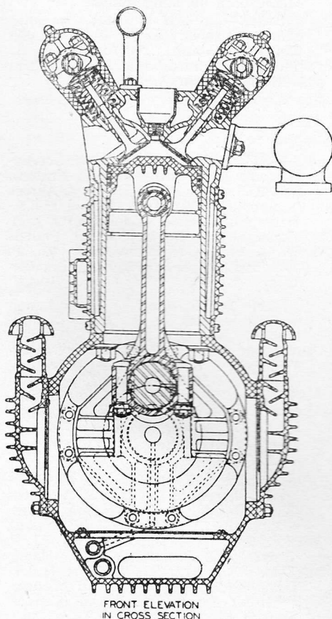
End section and construction details of the 4-cylinder, 4\frac{1}{2} -litre (270 cu. ins.) Offenhauser engine.
