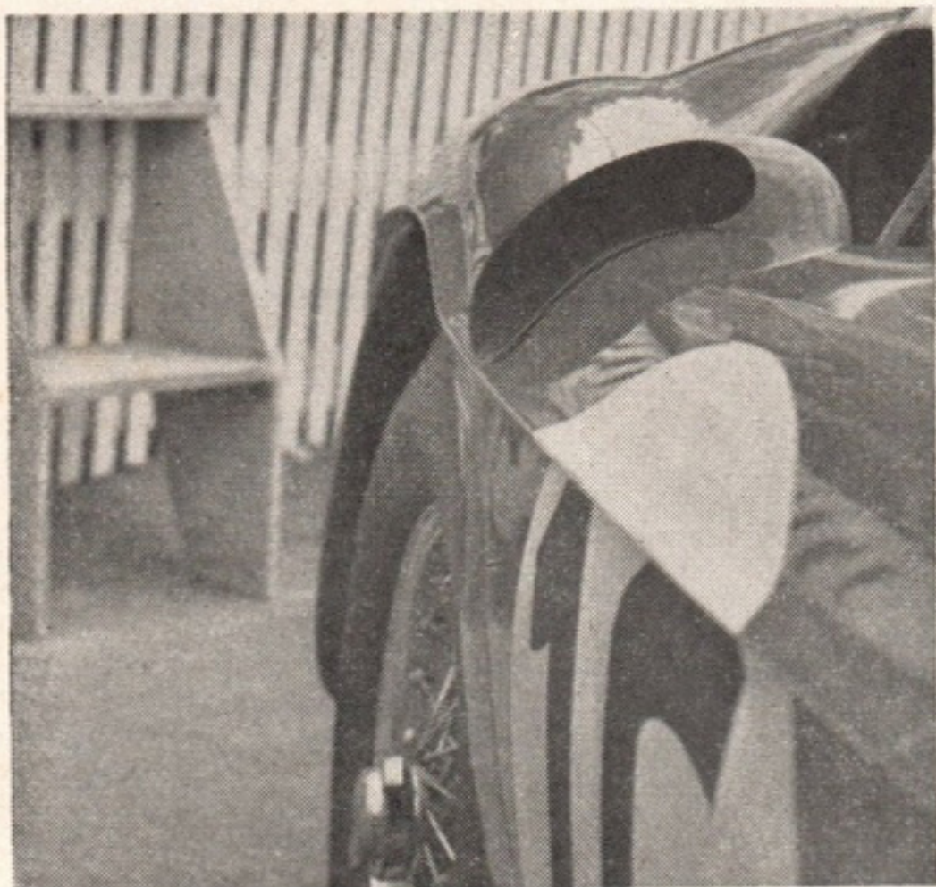
AID TO COOLING: (Above) A large intake on the wing of René Dreyfus's 4.1-litre Ferrari deflects air on to the rear brakes.
