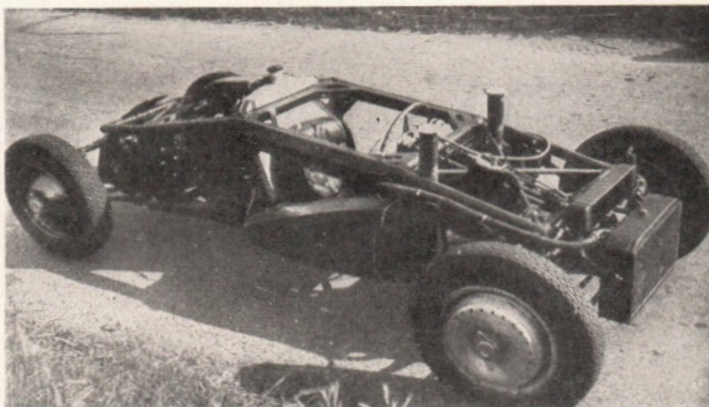
NEW FORMULA 2 CAR: The Lancia-Nardi will shortly be seen in G.P. events. It has a 2-litre, narrow V-6 Aurelia engine, rear-mounted in an ultra-lightweight frame constructed by Nardi-Danese. Suspension units, wheels and brakes are of Aurelia origin; the outside-mounted front brake drums are a prominent feature.
