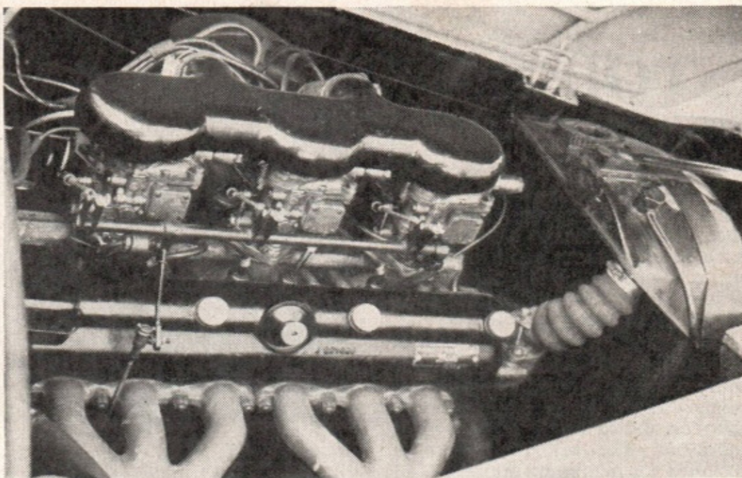
Three downdraught carburettors are used on the Bristol 401 engine, which, in modified form, is used on Frazer-Nash, Cooper-Bristol and E.R.A. The detail work is to the highest engineering standards.
