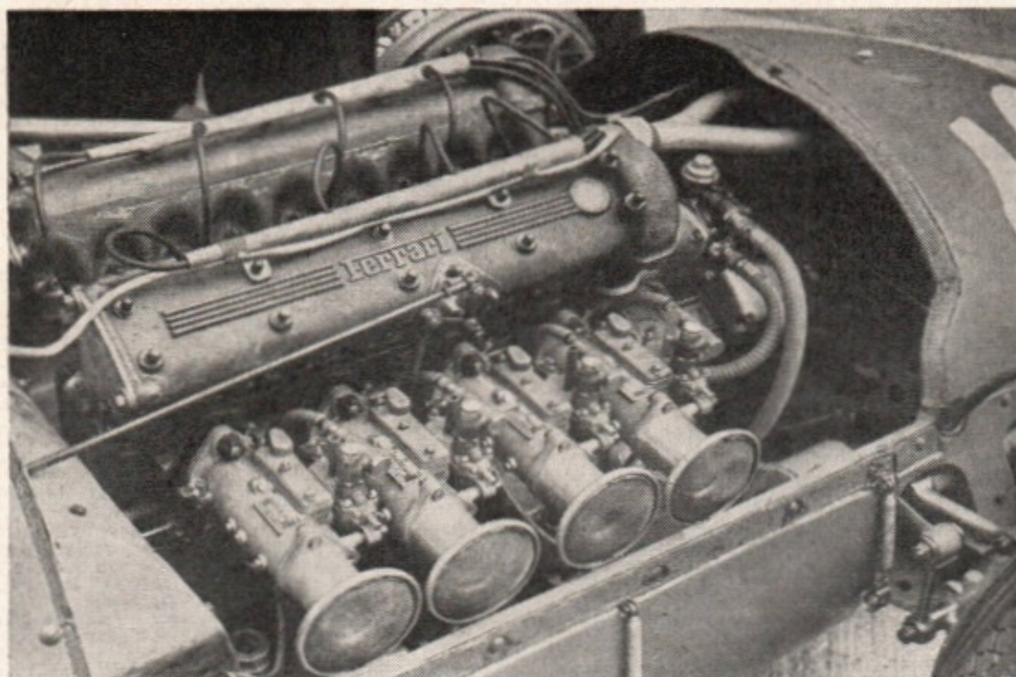
FORMIDABLE: Latest version of the 4-cylinder Ferrari has the engine moved back 3½ ins. in the frame, a single aircraft-type Marelli magneto at the front, stub exhausts and modified lay-out of the four 45 DOE Weber carburettors. It is reputed to develop over 190 b.h.p. at 7,500 r.p.m.
