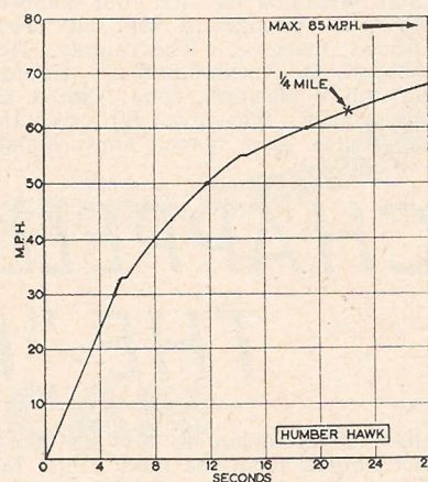
Acceleration Graph
