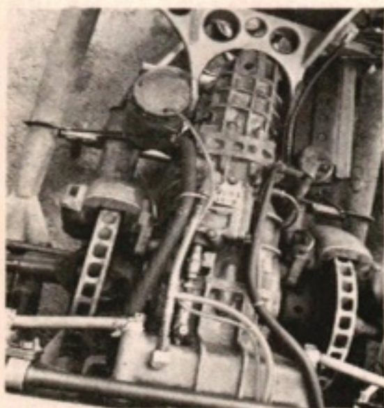
Brian Redman was down at Paul Ricard testing Ferrari's new G5 challenger recently. The bodywork is much smoother with an integral rear wing. Between the rollover bars is an airbox for the flat 12 engine (above). The F1 gearbox is used with inboard ventilated disc rear brakes (below left).
