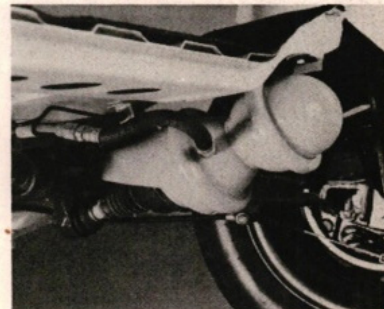
Hydragas rear suspension unit.
